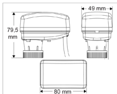
Overall Dimensions
